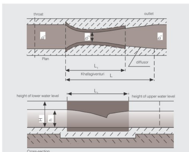
Dimensions of Khafagi-Venturi flumes
